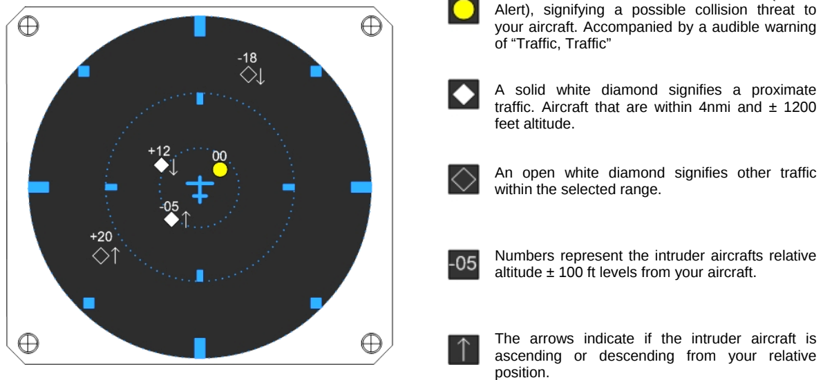
Typical TCAS I Display
